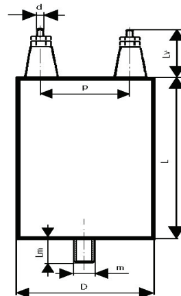
Tubular case type LV for HV capacitors
