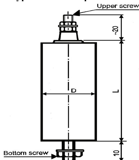
Tubular case type P for HV capacitors
