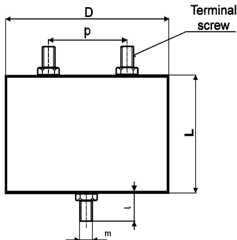
Tubular case type LV for HV capacitors
