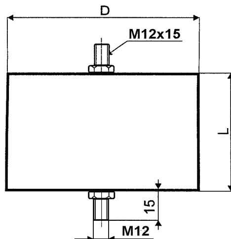
Tubular case, terminal screws, type P
