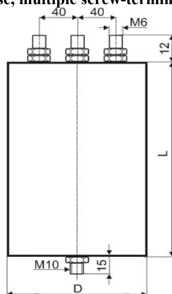
Tubular case, multiple screw-terminals, type L
